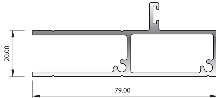
SECTION No. J007 1.022 kg/m P = 320.58
