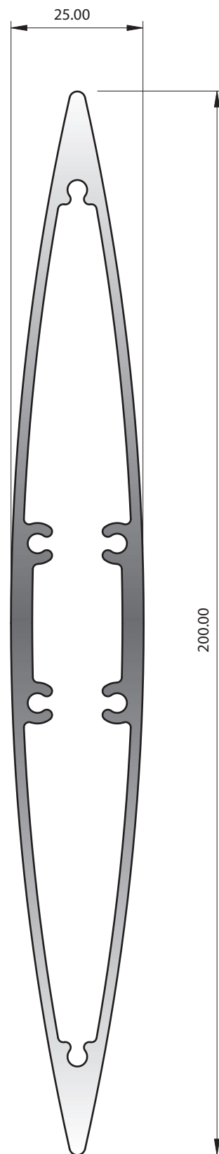
SECTION No. 32508 2.962 kg/m P = 406.69
