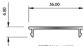
SECTION No. X537 0.179 kg/m P = 95.84
