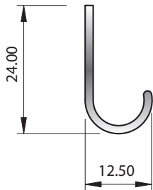
SECTION No. 6130 0.148 kg/m P = 76
