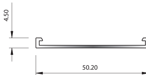
SECTION No. G338* 0.201 kg/m P = 121.67
